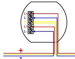
MG-1821.SCI INTELLIGENT ADDRESSABLE CARBONMONOXIDE GAS DETECTOR WITH SHORT CIRCUIT ISOLATOR
