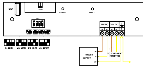
ML-1170.SCI ADD. BEAM DETECTOR TRANSMITTER
