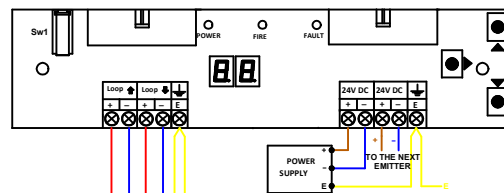
ML-1170.SCI ADD. BEAM DETECTOR EMITTER c/w SCI
