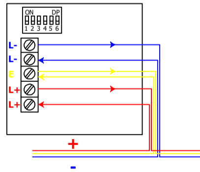
ML -1430.SCI INTELLIGENT ADDRESSABLE SOUNDER BEACON c/w SCI
