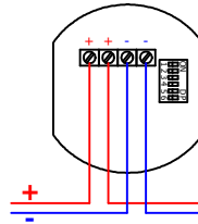
ML-2440 CONVENTIONAL SOUNDER ( IP 33 )
